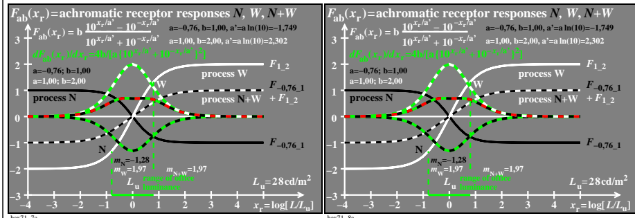
TUB-test chart hex7; Model of response functions F_{ab}(x_r) , processes N, W, N+W, and derivations Tangens hyperbolicus \tanh(x_r) and modified with e^{\pm x_r/a} and 10^{\pm x_r/a'} ; a=-0.76 & 1.00 ; a' = \ln(10)
