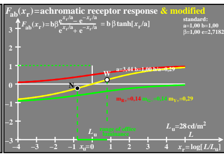
TUB-test chart heu0; TUBJND model response functions F_{ab}(x_r) , and derivation F'_{ab}(x_r) Receptor responses R_+ , G_- , Y_+ (left), and derivations R_+ , G_- (right) for different parameters a,b
