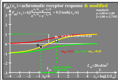
TUB-test chart heu0; TUBJND model response functions F_{ab}(x_r) , and derivation F'_{ab}(x_r) Receptor responses R_+ , G_- , Y_+ (left), and derivations R_+ , G_- (right) for different parameters a,b
