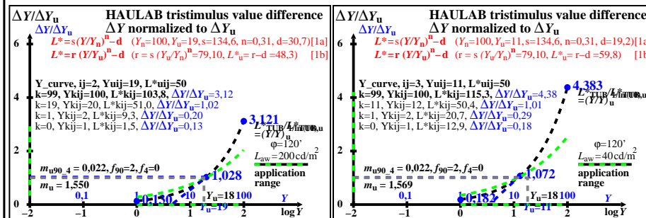
TUB-test chart heo6; HAULAB, adaptation W Lwu=300, 1000, 200, 40, Haubner (1980) & data lin[lighness L*, threshold ΔY, sensitivity ΔY / Y, contrast Y / ΔY, normalized for grey U]
