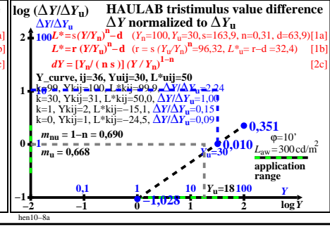
TUB-test chart hen1; HAULAB, sample-viewing angles 120' to 10', Haubner (1980) & data log[lightness L*, threshold ΔY, sensitivity ΔY/Y, contrast Y/ΔY, normalized for grey U]
