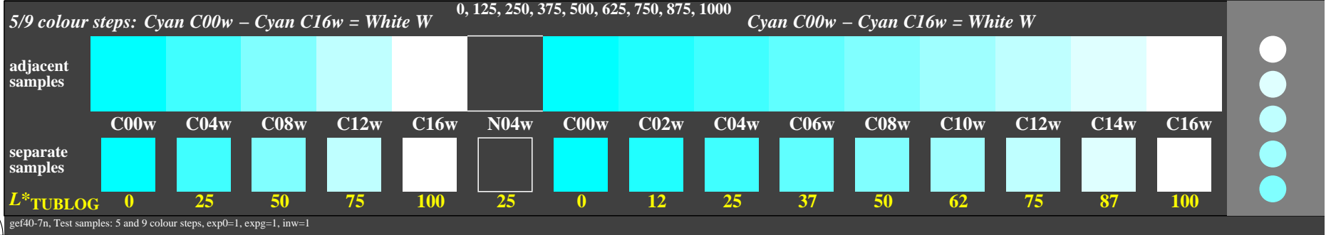
TUB-test chart gef4; Adjacent and separate colour samples for intervall scaling Evaluation of colour steps of the series C–W with 5 and 9 steps; surround dark Grey D=N04w
