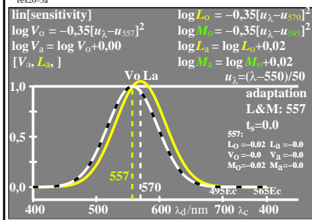
TUB-test chart eex2; sensitivity LMV->L/V & M/V, lin[thresholds]=0 & 0,04 lin[sensitivity] and lin[ratio], LMS-R21=570,545,557, adaptation 557
