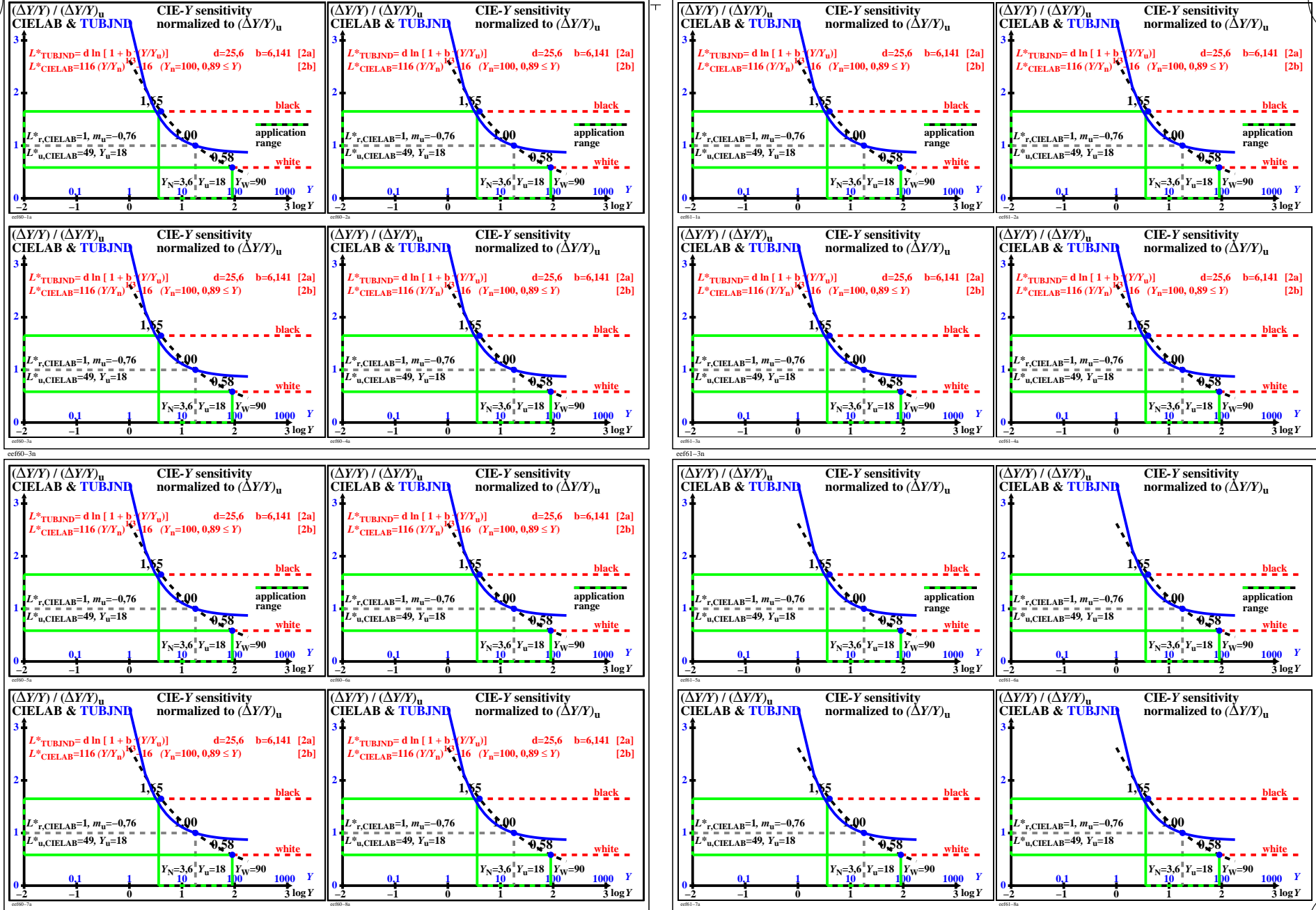
TUB-test chart eef6; Sensitivity (\Delta Y/Y) / (\Delta Y/Y)_u = f[\log(Y)] of colour spaces CIELAB & TUBJND, see ISO/CIE 11664-4 & CIE 230, many information (left), and less (right)
