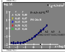
TUB-test chart TN64; threshold data Avramopoulos (89) 6.3cd/m²
