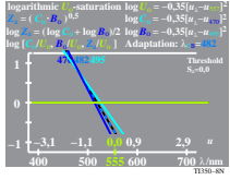
grafico TUB-TI35; colour vision and colorimetry cone sensitivity and saturation for distance \Delta\lambda=25
