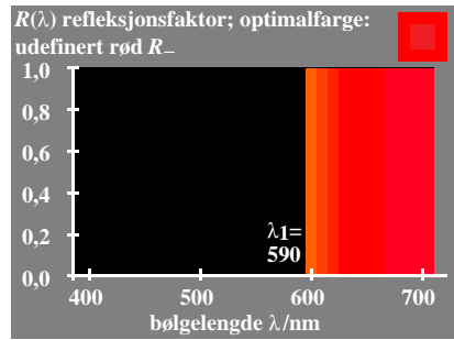
5-003030-L0 MN050-3N, B2_49_1
