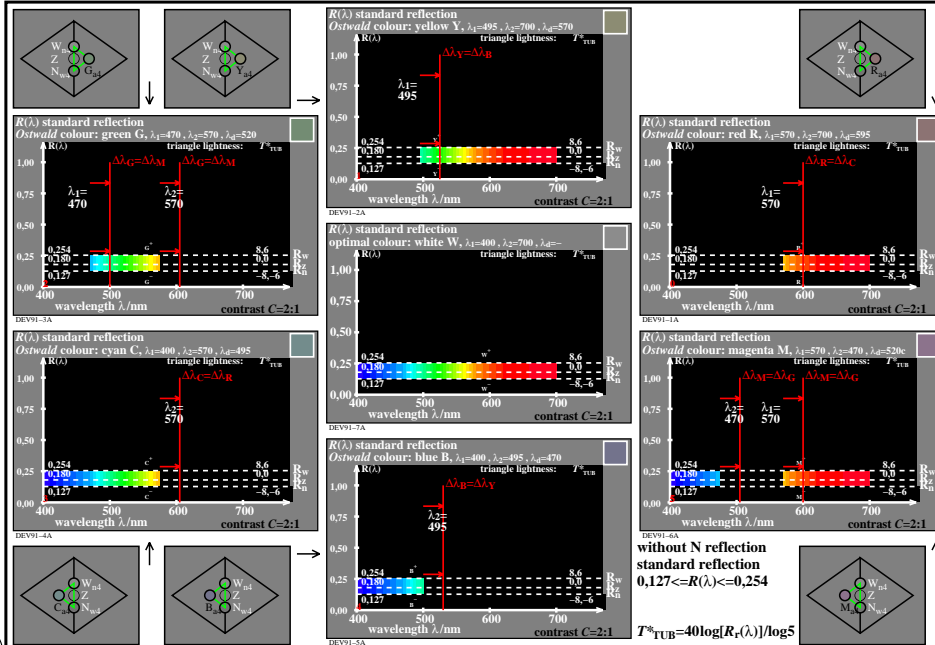
TUB-test chart DEV9; Wavelength ranges of 6 Ostwald colours, and white W Reflections R(\lambda) , R_r(\lambda) = R(\lambda)/0,18 , and R_s(\lambda) = \log[R_r(\lambda)] , hue threshold \Delta h_{A2B2} = 18 , C = 2:1
