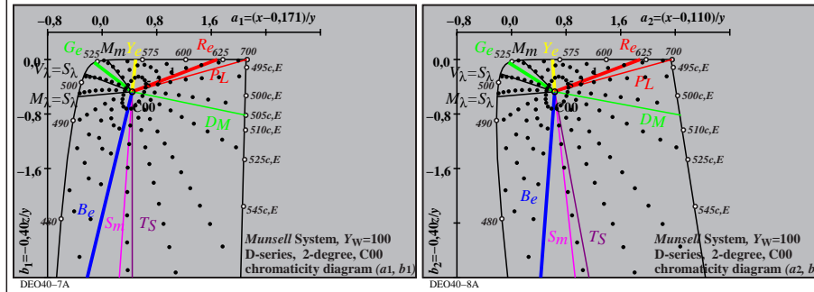
TUB-test chart DEO4; 2 degree observer; Illuminant C00, Munsell colour system lightness (Value) V_{Munsell}=2 , near L^*_{CIELAB}=20 , extrapolated (left) and samples (right)
