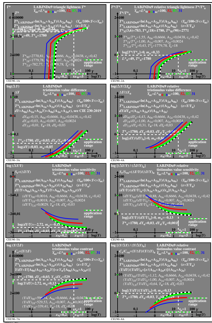
TUB-test chart CEU9; LABJNDu9, t^*(Y) & T^*(Y) , Y_{nc}=(Y \cdot L^*)_{WRGBnc} , c_x=0.43 , with more data Lightness, sensitivity and contrast, A_{0n}=0.6666, A_{1n}=0.007, A_{2n}=0.0024, A_{2u}=0.044
