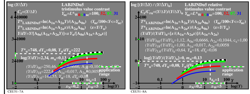
TUB-test chart CEU5; LABJNDu5, t^*(Y) & T^*(Y) , Y_{nc}=(Y \cdot L^*)_{WRGBnc} , c_x=1,00 , with more data Lightness, sensitivity and contrast, A_{0n}=0,6666 , A_{1n}=0,017 , A_{2n}=0,0058 , A_{2u}=0,104
