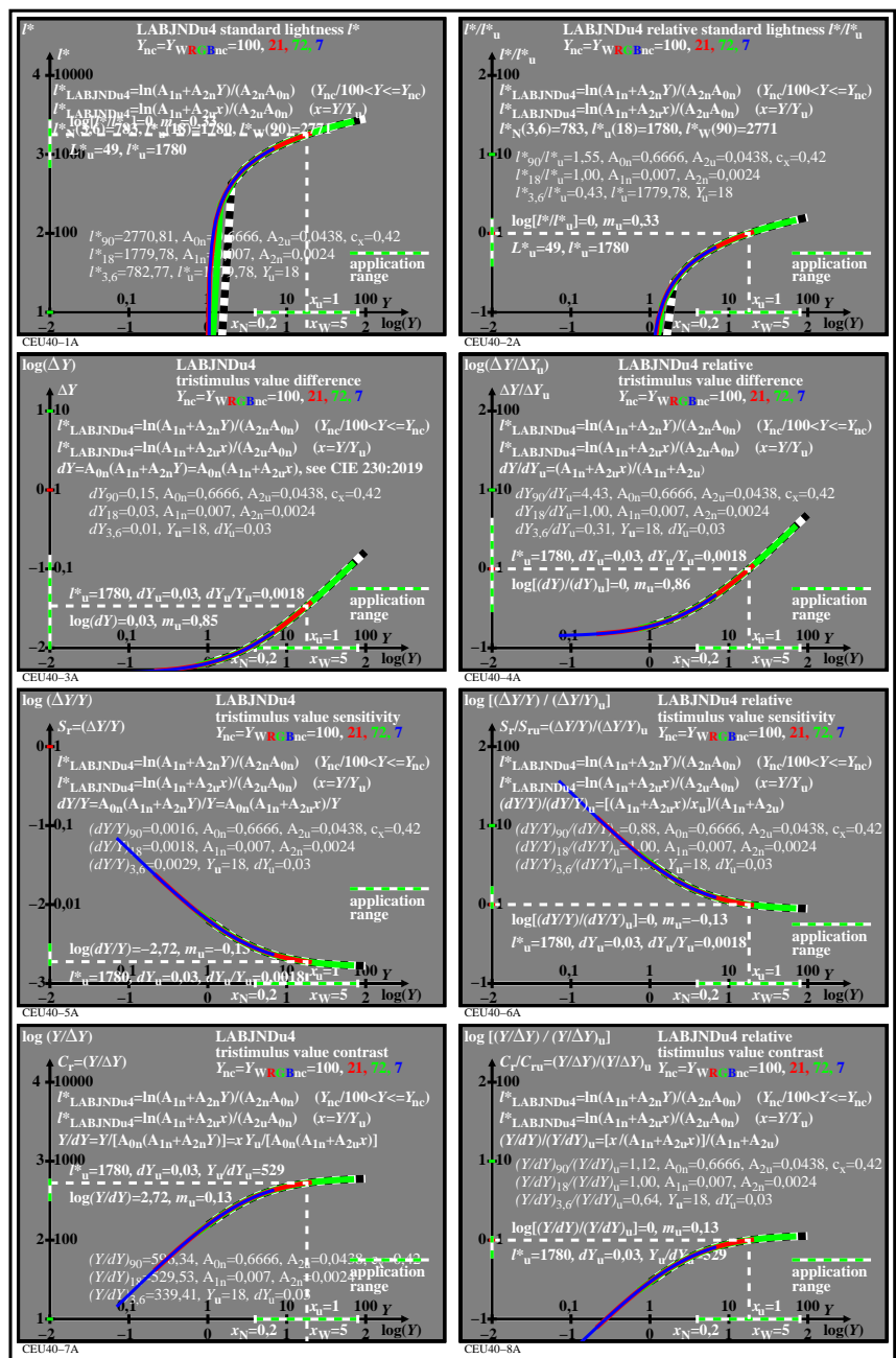
TUB-test chart CEU4; LABJNDu4, l^*(Y) & L^*(Y) , Y_{nc}=(Y \cdot L^*)_{W_{nc}} , c_x=0,43 , with more data Lightness, sensitivity and contrast, A_{0n}=0,6666 , A_{1n}=0,007 , A_{2n}=0,0024 , A_{2u}=0,044
