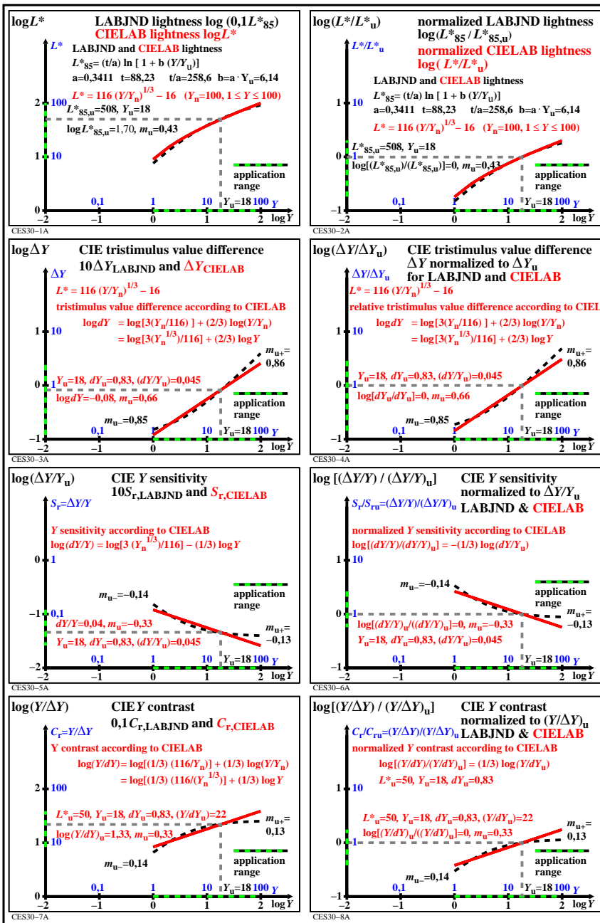
TUB-test chart CES3; Comparison of the LABJND and the CIELAB colour-difference formula \log[\text{lightness } L^*, \text{ threshold } \Delta Y, \text{ sensitivity } \Delta Y/Y, \text{ contrast } Y/\Delta Y, \text{ unnormalized and normalized}]
