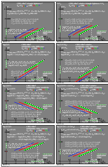
TUB-test chart BEX7; CIE LABu7, t^* & T^* for Y/Y_u with additional data, Y_{NC} = (Y \cdot L^*)_{WRGBnc} Absolute and relative lightness, sensitivity and contrast, S_{90} = 58.42, 1/\gamma = 1/2.5 = 0.40, D_N = 8.42
