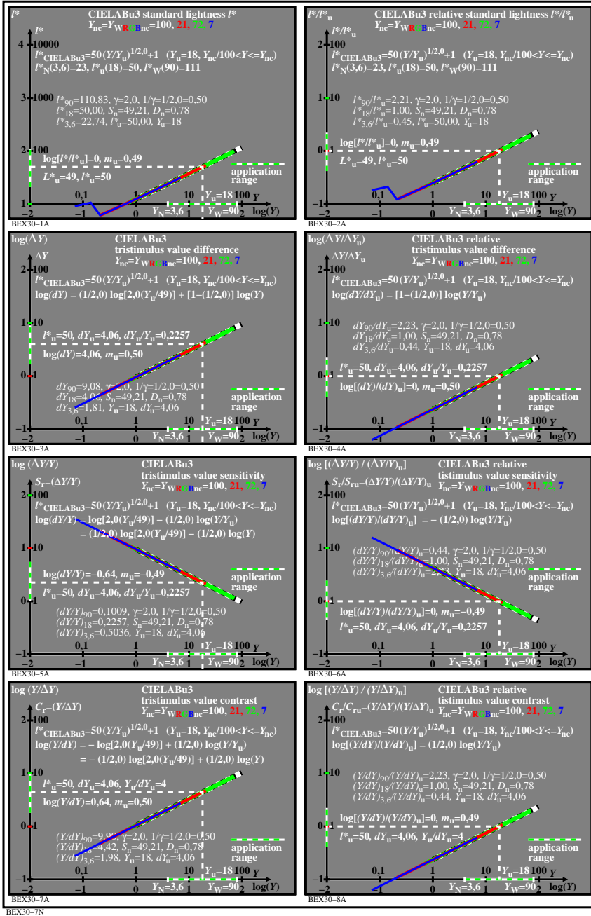
TUB-test chart BEX3; CIELABu3, l^* & L^* for Y/Y_u with additional data, Y_{nc}=(Y \cdot L^*)_{W_{nc}} Absolute and relative lightness, sensitivity and contrast, S_n=49,21 , 1/\gamma=1/2,0=0,50 , D_n=0,78
