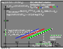
TUB-test chart BEW5; IECsRGBu5, t^* & T^* for Y/Y_n, Y_{nc} = (Y \cdot L^*)/W_{RGBnc} Absolute and relative lightness, sensitivity and contrast, S_n = 50, 00, 1/\gamma = 1/2.4 = 0.41
