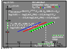
TUB-test chart BEW5; IECsRGBu5, t^* & T^* for Y/Y_n, Y_{nc} = (Y \cdot L^*)/W_{RGBnc} Absolute and relative lightness, sensitivity and contrast, S_n = 50, 00, 1/\gamma = 1/2.4 = 0.41
