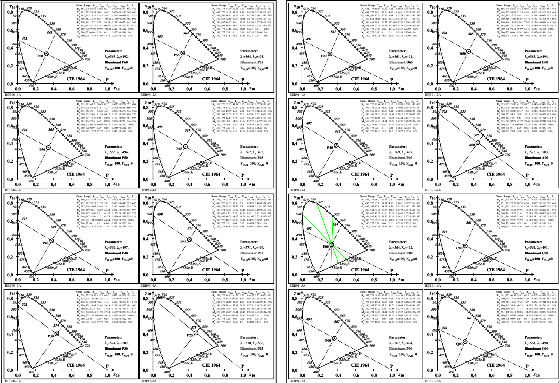
TUB-test chart BEB9; 6 Ostwald optimal colours for 8 illuminants Pxx (left) and Dxx (right), (x_{10}, y_{10})_{400,700} , lines separate wavelength ranges of Ostwald optimal colours
