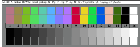
AE140-7, Picture D3Wdd: 14 CIE-test colours and 2 + 16 grey steps (sf); rgb/cmy0 \rightarrow rgb_{d4} setrgbcolor
