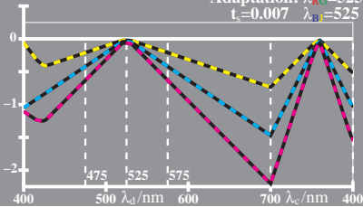
WE981-1, Change of PDT (LMS) in colour vision; Adaptation
