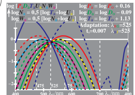
WE960-1, Change of PDT (LMS) in colour vision; Adaptation
