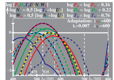
WE960-7, Change of PDT (LMS) in colour vision; Adaptation
