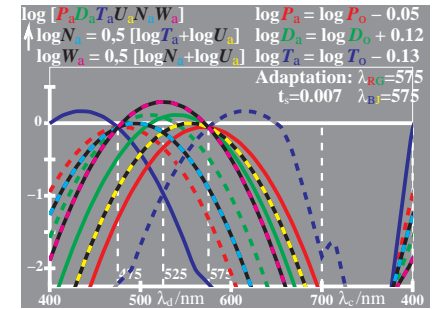
WE960-3, Change of PDT (LMS) in colour vision; Adaptation
