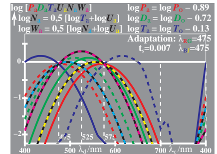
WE960-5, Change of PDT (LMS) in colour vision; Adaptation
