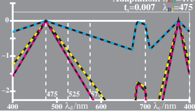
WE931-5, Change of PDT (LMS) in colour vision; Adaptation
