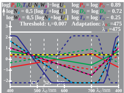
WE920-6, Change of PDT (LMS) in colour vision; Adaptation
