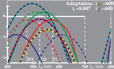
WE910-7, Change of PDT (LMS) in colour vision; Adaptation
