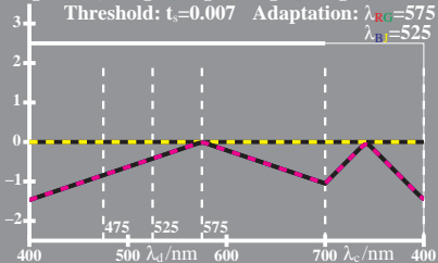
WE851-3, Change of PDT (LMS) in colour vision; Adaptation
