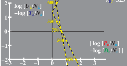
WE841-4, Change of PDT (LMS) in colour vision; Adaptation
