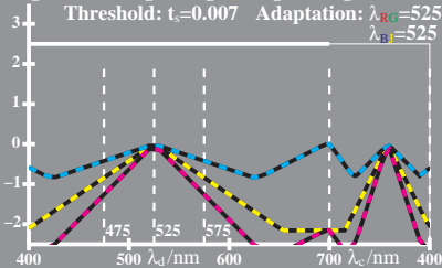
WE841-1, Change of PDT (LMS) in colour vision; Adaptation
