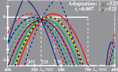
WE820-1, Change of PDT (LMS) in colour vision; Adaptation
