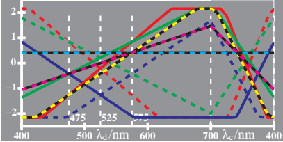
WE811-7, Change of PDT (LMS) in colour vision; Adaptation
