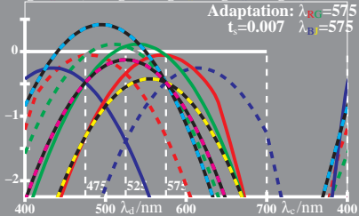
WE810-7, Change of PDT (LMS) in colour vision; Adaptation
