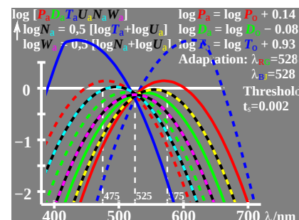
WE771-3, Change of PDT (LMS) in colour vision; Adaptation
