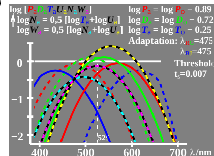
WE770-1, Change of PDT (LMS) in colour vision; Adaptation
