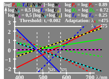
WE771-2, Change of PDT (LMS) in colour vision; Adaptation
