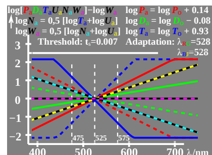
WE770-4, Change of PDT (LMS) in colour vision; Adaptation
