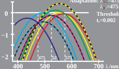
WE761-1, Change of LMS in colour vision; Adaptation
