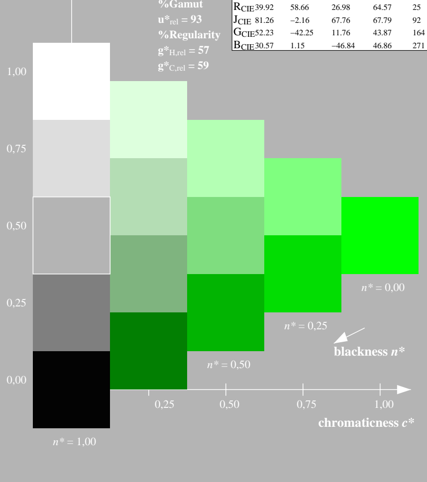
5 step scales for constant CIELAB hue 151/360 = 0.419 (right)
