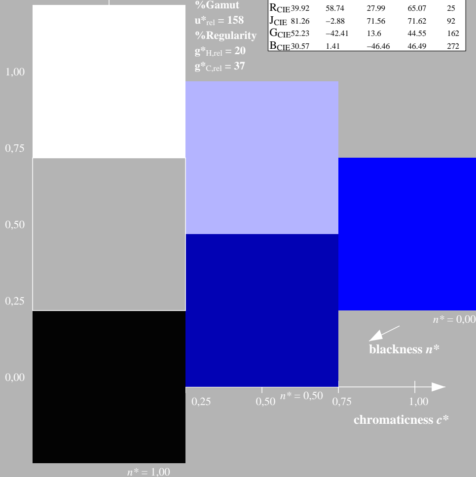
NE850-7, 3 step scales for constant CIELAB hue 306/360 = 0.851 (left)
