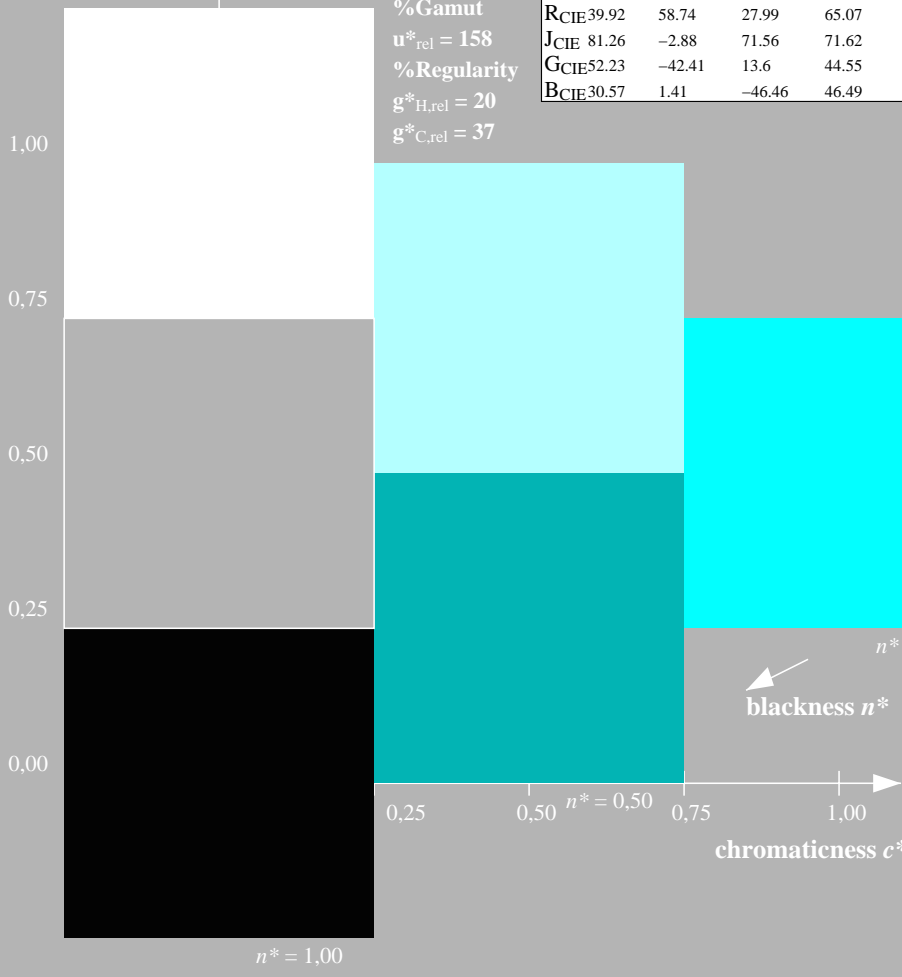
NE850-7, 3 step scales for constant CIELAB hue 196/360 = 0.545 (left)
