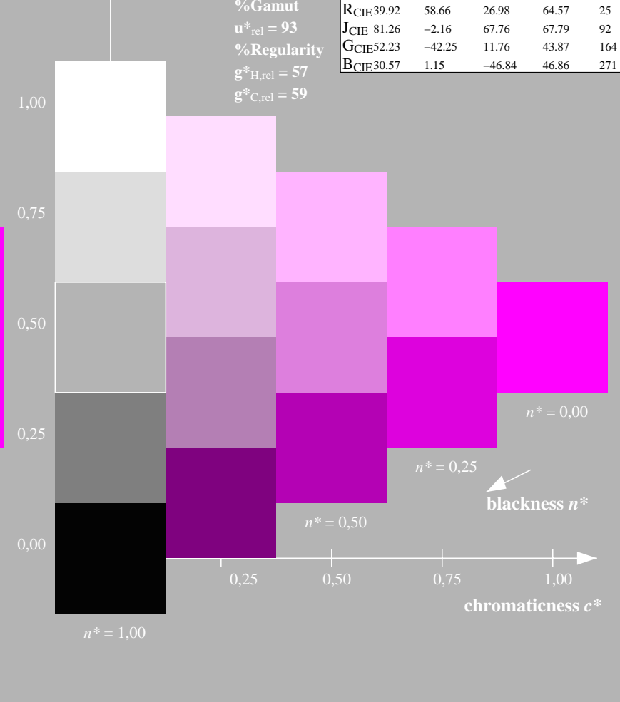
5 step scales for constant CIELAB hue 354/360 = 0.982 (right)
