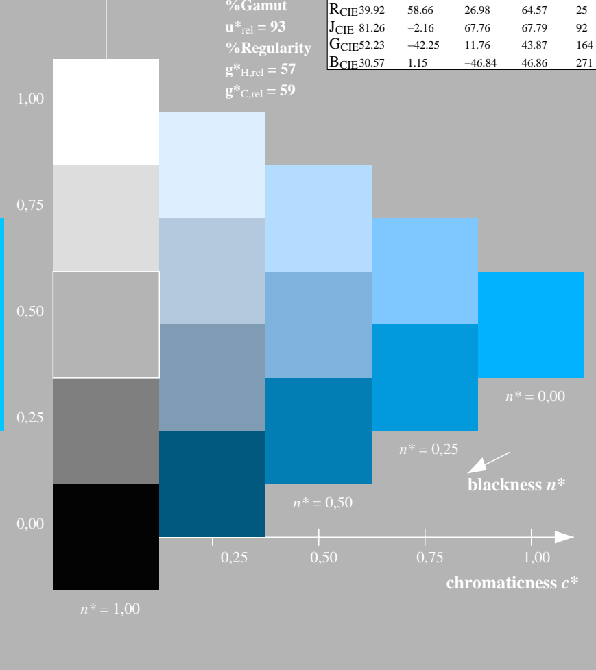
5 step scales for constant CIELAB hue 271/360 = 0.754 (right)
