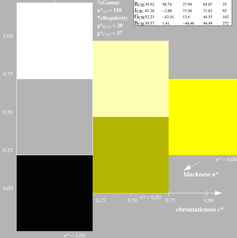
NE850-7, 3 step scales for constant CIELAB hue 103/360 = 0.286 (left)
