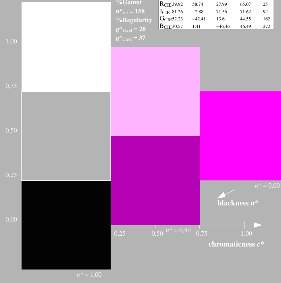
NE850-7, 3 step scales for constant CIELAB hue 328/360 = 0.912 (left)
