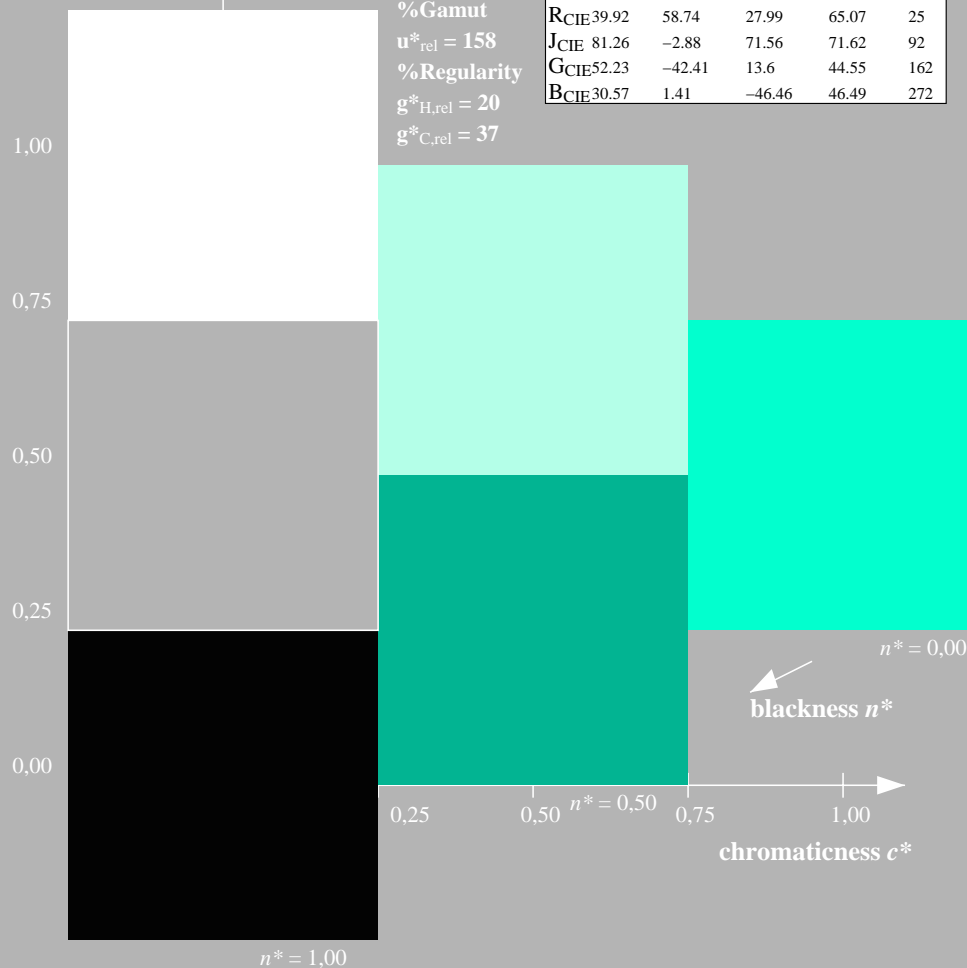
NE850-7, 3 step scales for constant CIELAB hue 162/360 = 0.451 (left)
