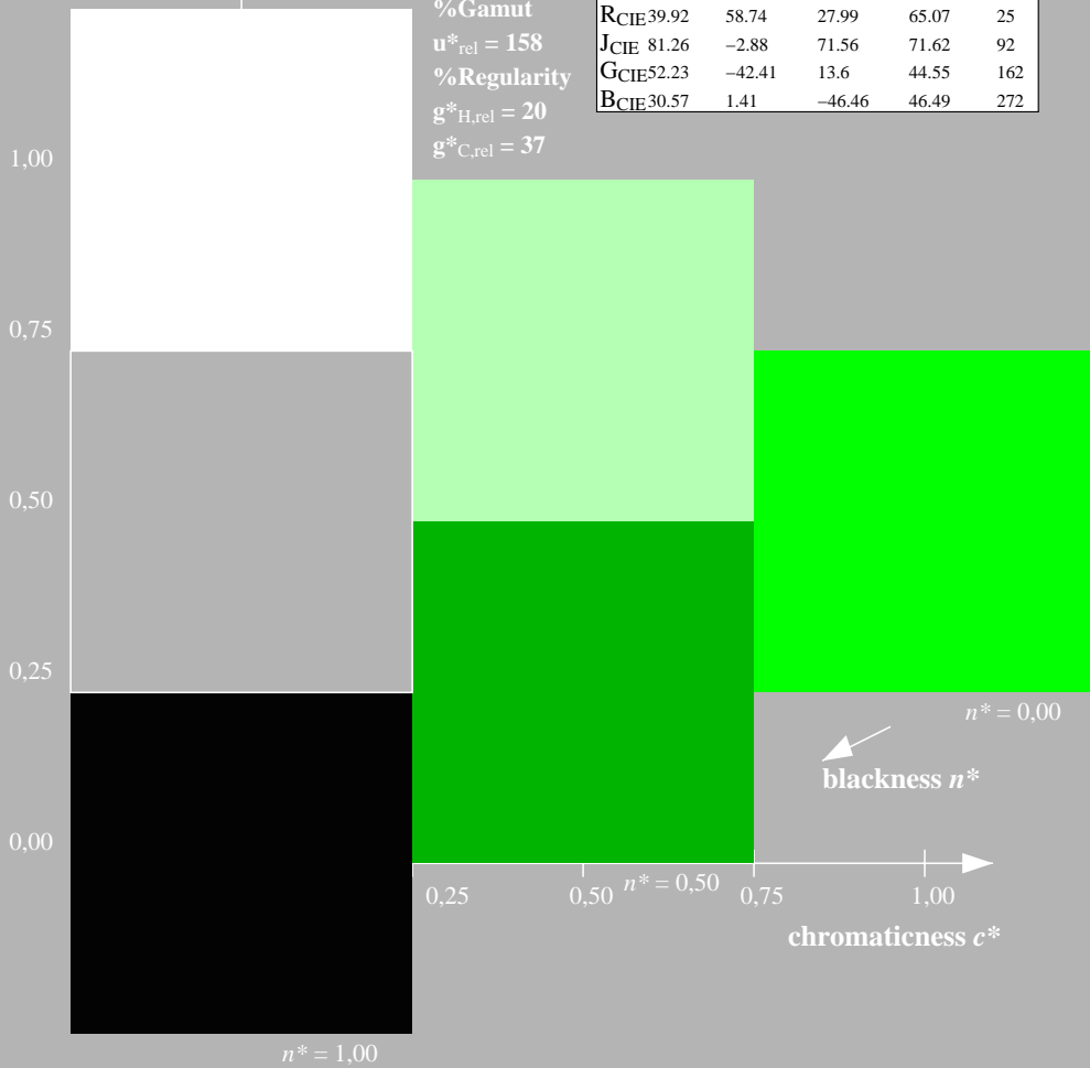
NE850-7, 3 step scales for constant CIELAB hue 136/360 = 0.378 (left)
