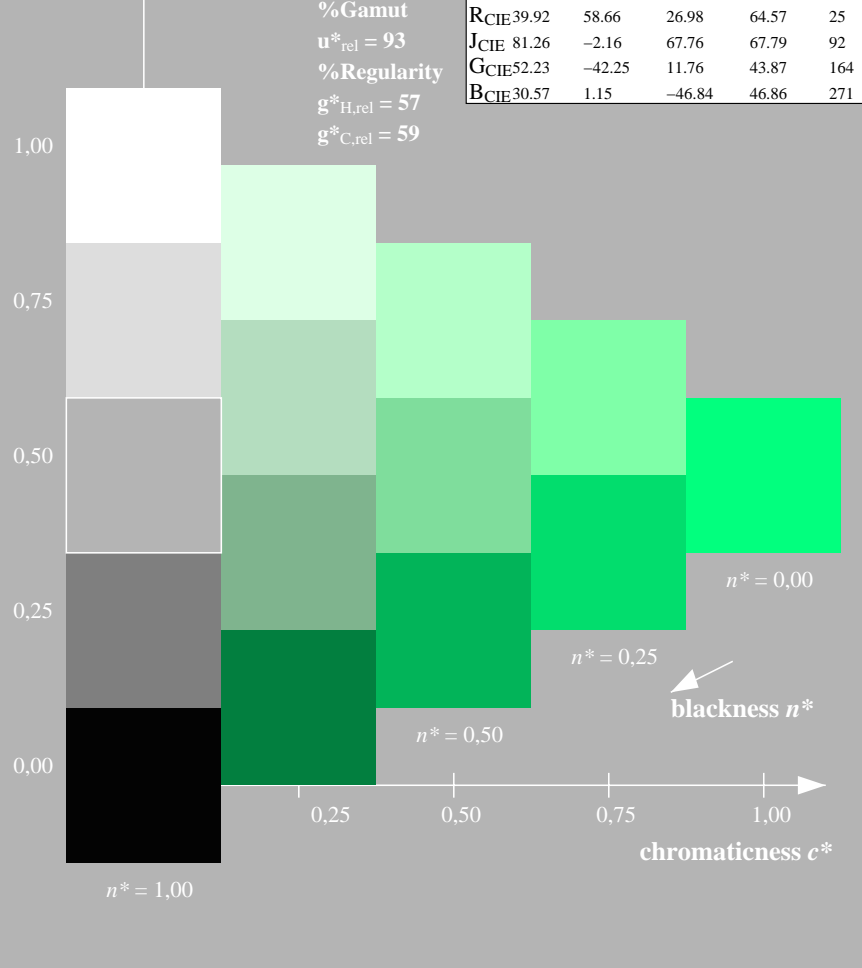
5 step scales for constant CIELAB hue 164/360 = 0.457 (right)
