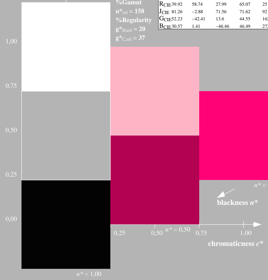
NE850-7, 3 step scales for constant CIELAB hue 25/360 = 0.071 (left)
