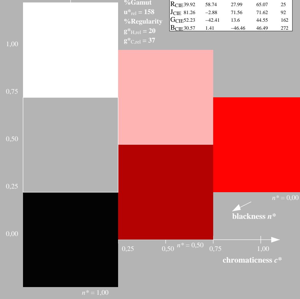
NE850-7, 3 step scales for constant CIELAB hue 40/360 = 0.111 (left)
