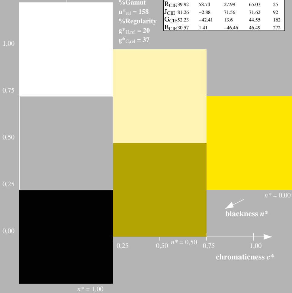
NE850-7, 3 step scales for constant CIELAB hue 92/360 = 0.256 (left)
