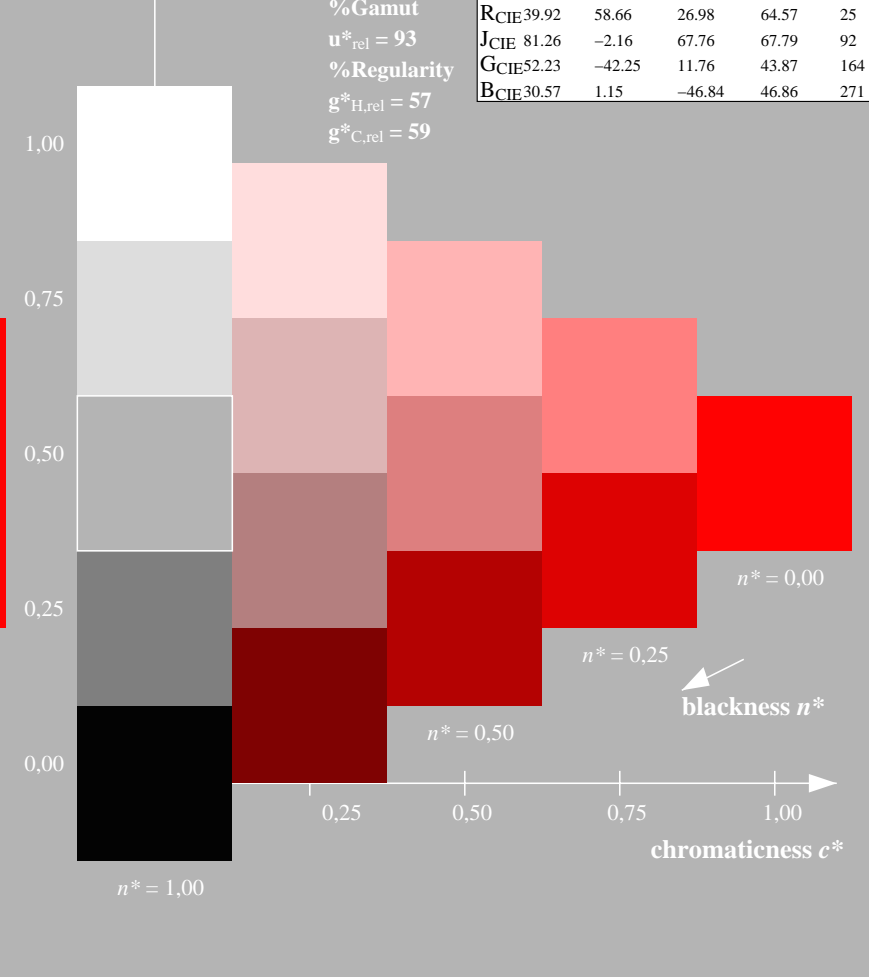
5 step scales for constant CIELAB hue 38/360 = 0.105 (right)
