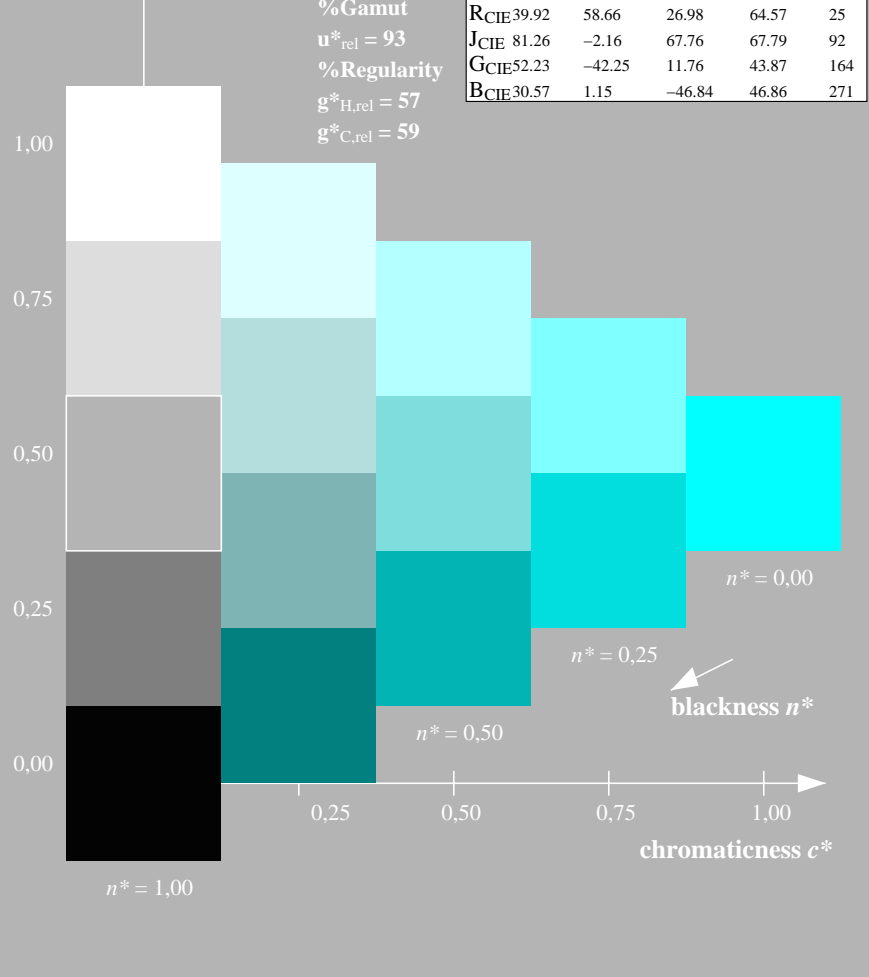
5 step scales for constant CIELAB hue 236/360 = 0.656 (right)
