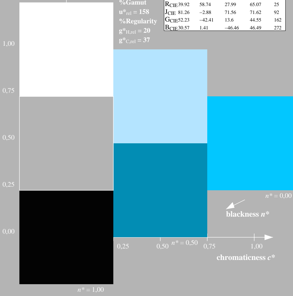
NE850-7, 3 step scales for constant CIELAB hue 272/360 = 0.755 (left)
