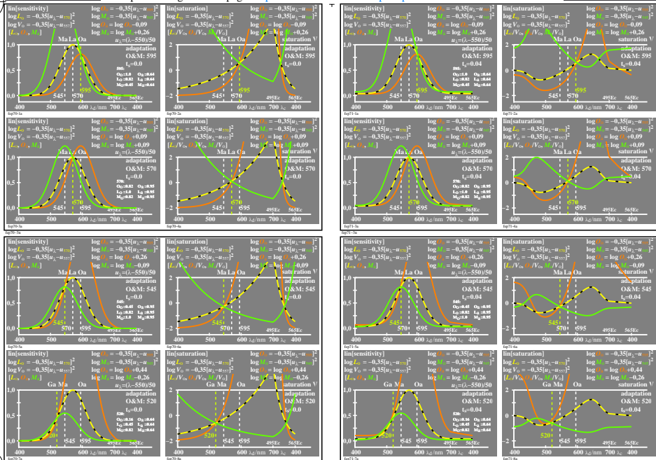
TUB-test chart fep7: sensitivity LMO→L/V & O/V, lin[thresholds]=0 & 0,04 lin[sensitivity] and lin[ratio], LMS-R24, 4 adaptations: 595,570,545,520
