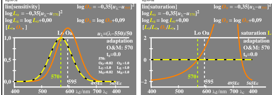
TUB-test chart fep3; sensitivity LMO \rightarrow M/L & O/L, lin[thresholds]=0 & 0,04 lin[sensitivity] and lin[ratio], LMS-R24=595,570,545, adaptation 570
