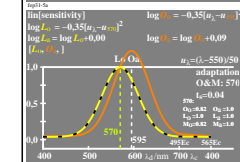
TUB-test chart fep3; sensitivity LMO->M/L & O/L, lin[thresholds]=0 & 0,04 lin[sensitivity] and lin[ratio], LMS-R24=595,570,545, adaptation 570
