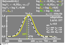
TUB-test chart fep2: sensitivity LMV->L/V & M/V, lin[thresholds]=0 & 0.04 lin[sensitivity] and lin[ratio], LMS-R24=570,545,557, adaptation 557
