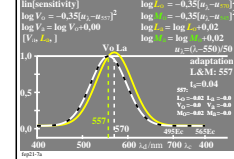
TUB-test chart fep2: sensitivity LMV->L/V & M/V, lin[thresholds]=0 & 0.04 lin[sensitivity] and lin[ratio], LMS-R24=570,545,557, adaptation 557
