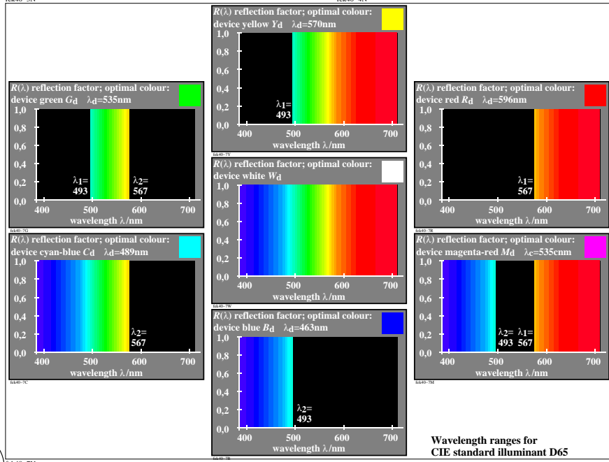
TUB-test chart fek4; Additive colour mixture; spectral mixture to optimal colour of Ostwald , ideal projector colours, colour mixture in colour television for D65
