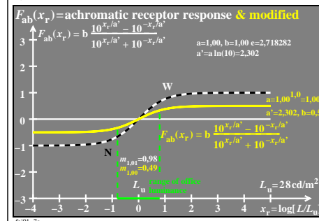
TUB-test chart fej0; Model of achromatic response functions F_{ab}(x_r) , visual processes N, W, N+W Tangens hyperbolicus \tanh(x_r) and modified with e^{x_r/a} and 10^{x_r/a} ; a' = a \ln(10)
