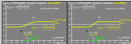
TUB-test chart fej0; Model of achromatic response functions F_{ab}(x_r) , visual processes N , W , N+W Tangens hyperbolicus \tanh(x_r) and modified with e^{x_r/a} and 10^{x_r/b} ; a = a \ln(10)
