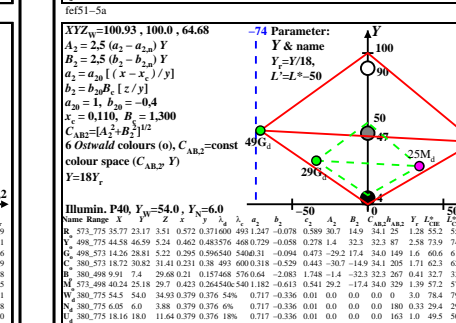
TUB-test chart fe5; 6 Ostwald optimal colours, Y_W = 100.0 , D65, D50, P40, A00, CIE-02-degree, Y_B constant chromatic value C_{A,B,2} , contrasts C \Rightarrow 288:1(100:0) , 25:1(90:3.6) , 16:1(72:4.5) , 9:1(54:6) , L^*
