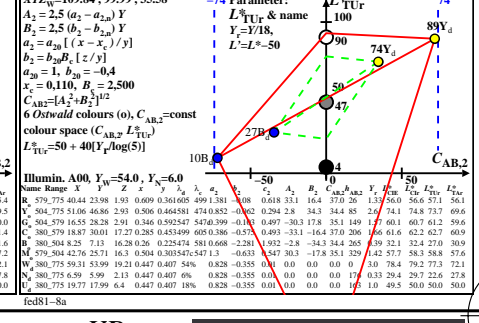
TUB-test chart fed8; Ostwald optimal colours, Yw=100.0, D65, D50, P40, A00, CIE-02-degree, YB constant chromatic value CAB2, contrast C=>288:1 (100:0), 25:1 (90:3.6), 16:1 (72:4.5), 9:1 (54:6), L*
