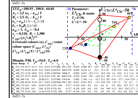
TUB-test chart fed2; Ostwald optimal colours, Y_w=100 , D65, D50, P40, A00, CIE-02-degree, Y_B constant chromatic value CAB2, contrasts C=>288:1 (100:0), 25:1 (90:3.6), 16:1 (72:4.5), 9:1 (54:6), L^*
