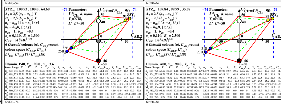
TUB-test chart fed2; Ostwald optimal colours, Y_w=100 , D65, D50, P40, A00, CIE-02-degree, Y_B constant chromatic value CAB2, contrasts C=>288:1 (100:0), 25:1 (90:3.6), 16:1 (72:4.5), 9:1 (54:6), L^*
