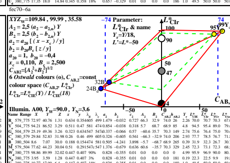
TUB-test chart fec7; Ostwald optimal colours, Yw=100, D65, D50, P40, A00, CIE-02-degree, YB constant chromatic value CAB2=>288:1(100:0), 25:1(90:3.6), 16:1(72:4.5), 9:1(54:6), L*
