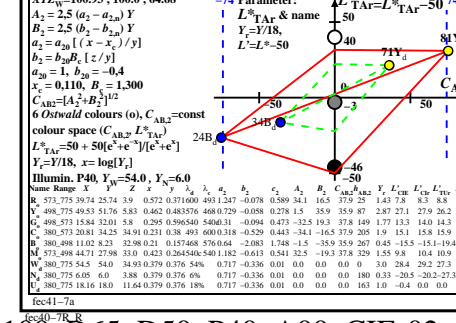
TUB-test chart fec4; Ostwald optimal colours, Y_W=100, D65, D50, P40, A00, CIE-02 -equivalent, Y_B constant chromatic value C_{AB,2} ; 25:1(90:3.6), 16:1(72:4.5), 9:1(54:6), L^*
