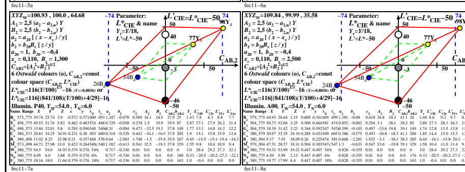
TUB-test chart fec1; Ostwald optimal colours, Yw=100, D65, D50, P40, A00, CIE-02-degree, YB constant chromatic value CAB2, C=>288:1(100:0), 25:1(90:3.6), 16:1(72:4.5), 9:1(54:6), L'
