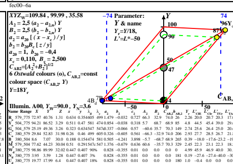
TUB-test chart fec0; Ostwald optimal colours, Y_W=100 , D65, D50, P40, A00, CIE-02-degree, YB constant chromatic value CAB_2 \Rightarrow 288:1(100:0) , 25:1(90:3.6), 16:1(72:4.5), 9:1(54:6), L^*=187
