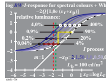
TUB-test chart feb5: Colour vision and physiology; reflection range for surface colours Physiological responses in colour vision as function of luminance and chromaticity
